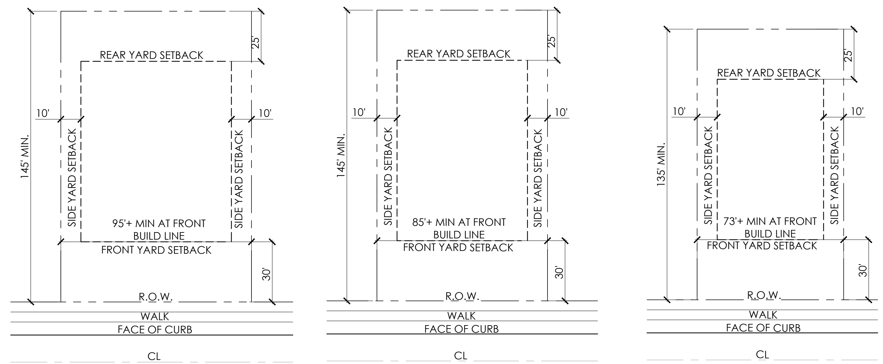
1 TYP. 95'x145' LOT CONFIGURATION SCALE: 1" = 30'
